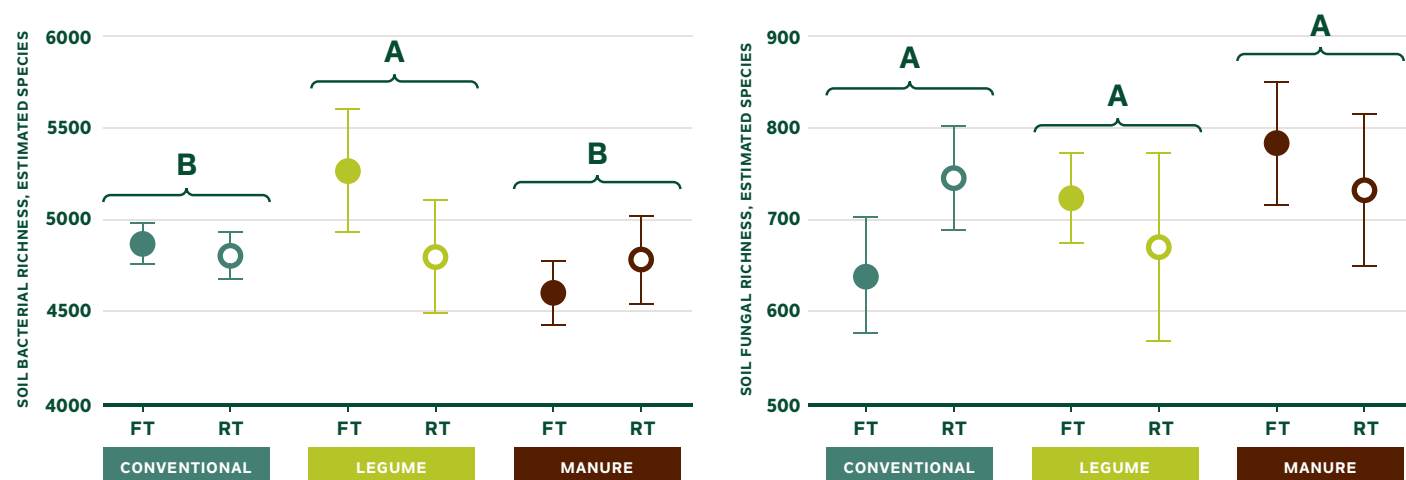
Figure 6 (Left) Soil (0–30 cm) bacterial richness and (Right) fungal richness of each of the systems in the Farming Systems Trial in 2019.
