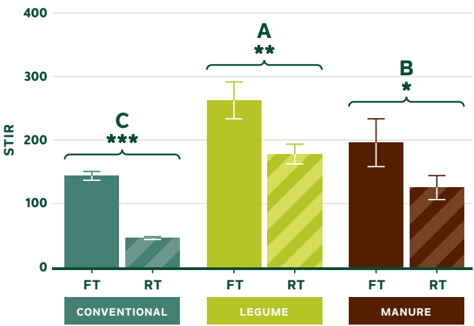
Figure 1 Average annual Soil Tillage Intensity Rating (STIR) of each of the systems in the Farming Systems Trial from 2008–2020. The STIR is a rating system created by USDA NRCS to measure overall soil disturbance. It accounts for tillage type, depth of tillage operation, operational speed of tillage equipment, and percentage of the soil surface area disturbed.
