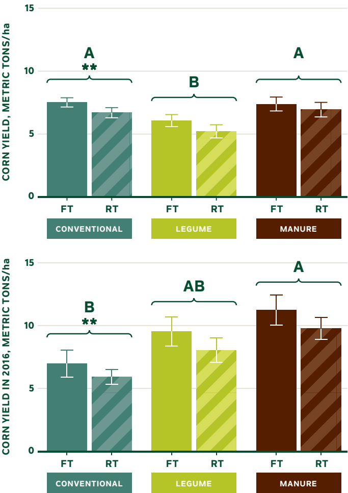
Figure 11 Average corn yield of each of the systems in the Farming Systems Trial from 2008–2020 (Top) and corn yield in 2016 (Bottom) which was an especially dry season.
