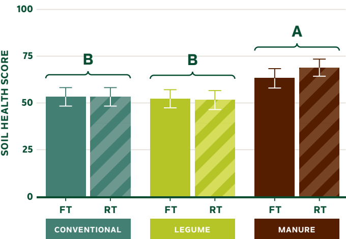
Figure 10 Cornell comprehensive assessment of soil health (CASH) score of each of the systems in the Farming Systems Trial in 2019 and 2020.
