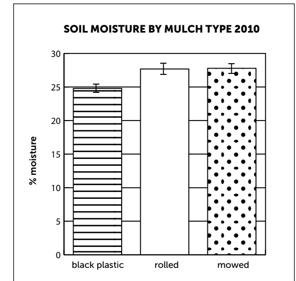
This chart demonstrates the trend observed across the soil moisture data: beds covered with black plastic mulch generally had lower moisture than the mowed and rolled beds. While this pattern was observed on many of the sampling dates, it was not always the case.
