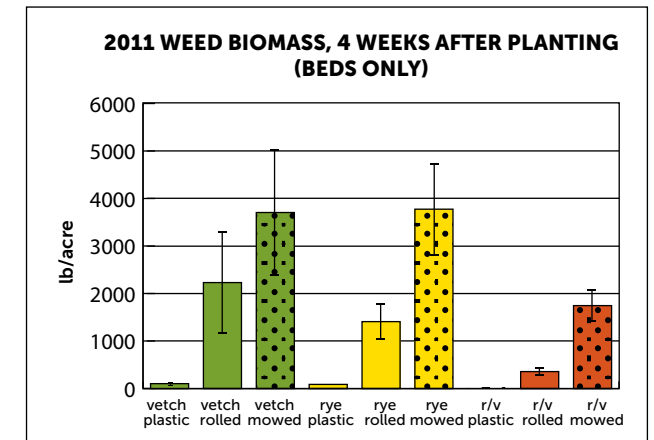
This chart shows the weed biomass in 2011, measured four weeks after planting, in all treatments. These values represent weeds growing within the beds only (paths excluded).
