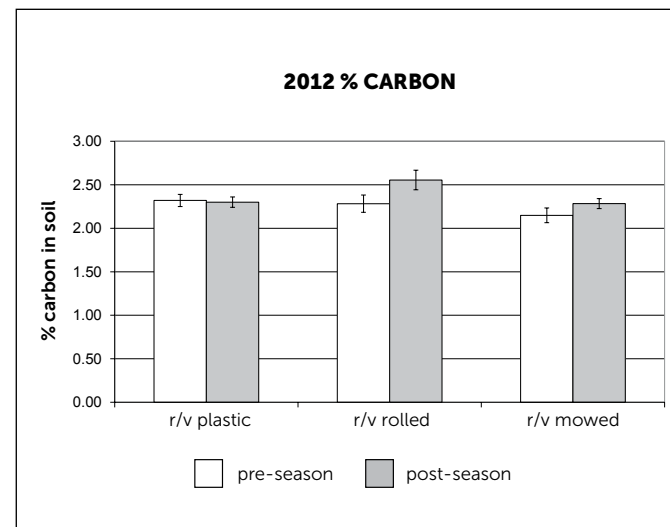
This chart shows the percent of carbon in the soils at the Rodale Institute test site pre- and post-season in 2012. Only the rye/vetch treatments are shown here, as there were no significant changes in the percent of carbon in either of vetch or rye singly.
