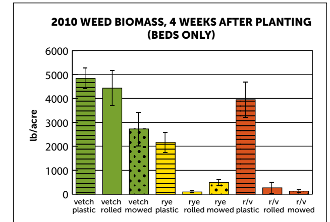
This chart shows the weed biomass in 2010, measured four weeks after planting, in all treatments. These values represent weeds growing within the beds only (paths excluded).
