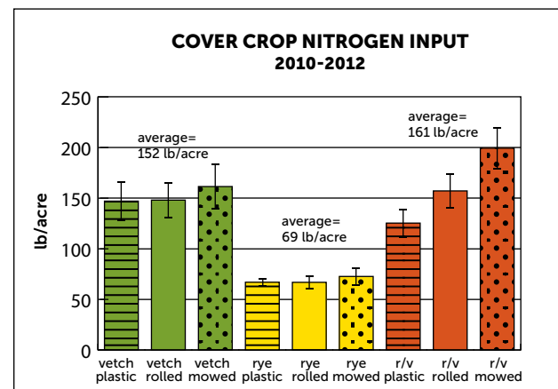
This chart shows the average nitrogen input from cover crops in each of the nine treatments. The values here are the averages from 2010, 2011, and 2012.
