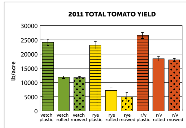
These charts show the total tomato yields in 2010 and 2011. Notice the variation between the two years: in 2010, the cover crop mulches outperformed the black plastic treatments, and in 2011 the pattern was reversed.
