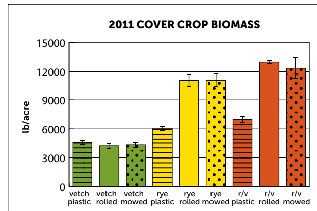
This chart shows the cover crop biomass in all treatments in 2011, measured just before cover crop termination. (Error bars represent standard errors.)
