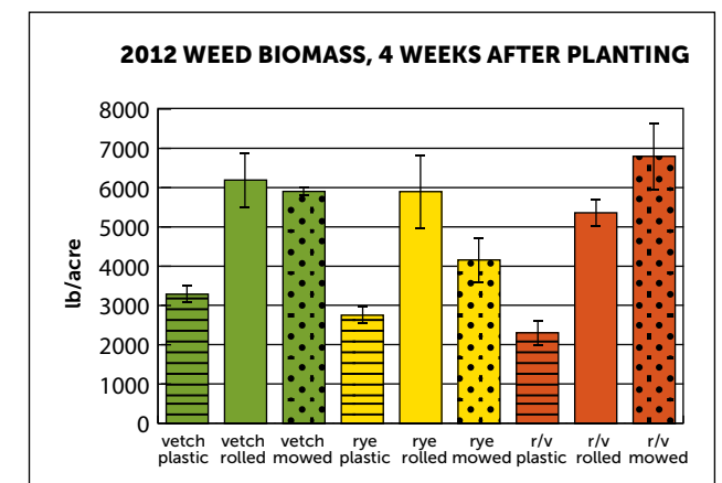
This chart shows the weed biomass in 2012, measured four weeks after planting, in all treatments. These values represent weeds growing within the beds and paths.
