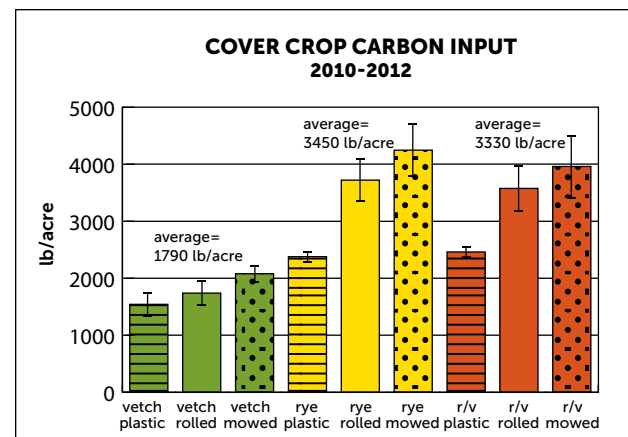
This chart shows the average carbon input from cover crops in each of the nine treatments. The values here are the averages from 2010, 2011, and 2012.
